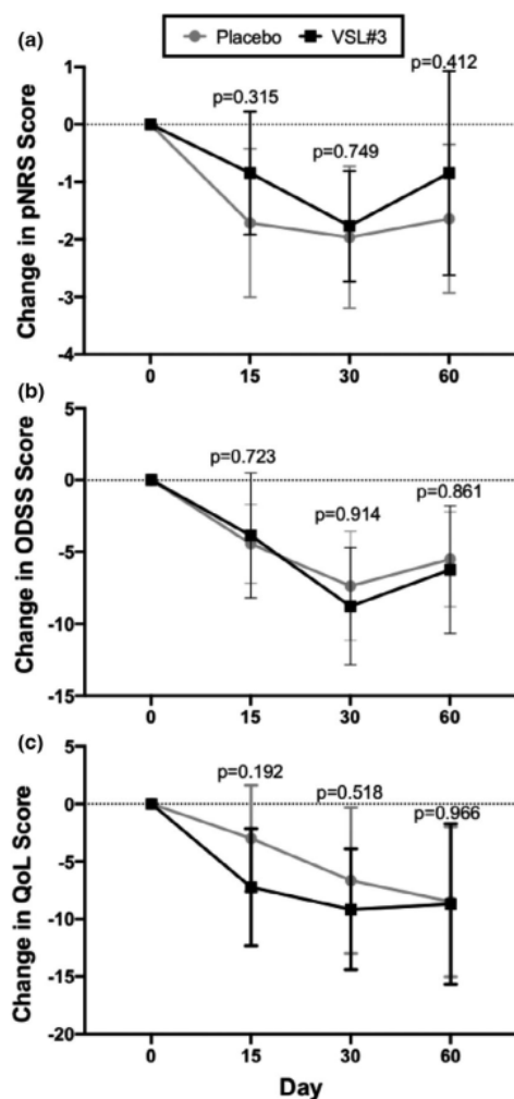
FIGURE 2 Alteration in clinical scores compared with baseline measurements over the trial period. Mean change in (a) pNRS, (b) ODSS and (c) QoL scores. p-values are from a comparison of randomised groups adjusting for the baseline score. Placebo group n = 14, VSL#3 group n = 13, Mean \pm 95% CI
